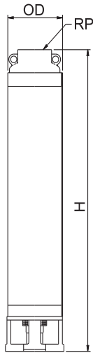
DIMENSIONS & WEIGHT
